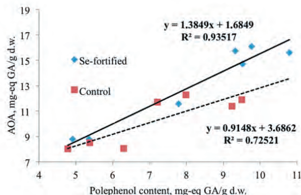
Fig.1. Relationship between AOA and polyphenol content in Allium seeds sprouts fortified ( r=+0.97 ; P<0.001 ) and non fortified ( r=+0.85 ; P<0.004 ) with selenium
